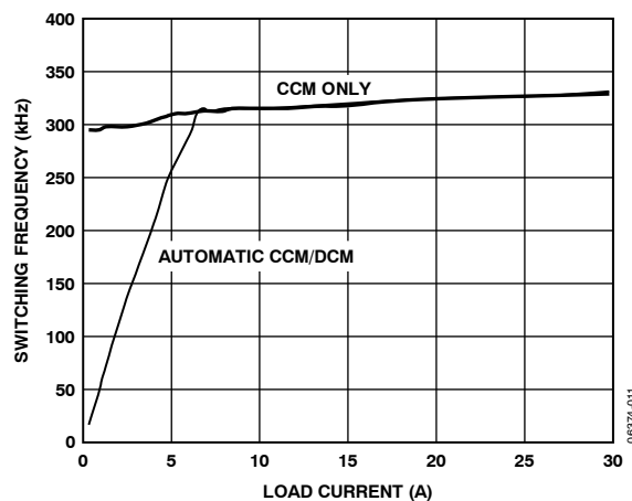
Figure 11. Switching Frequency vs. Load Current in RPM
