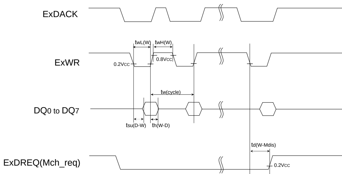
Fig. 176 Timing chart (6)
