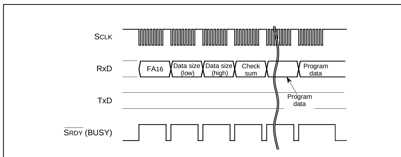
Fig. 160 Timing for download
