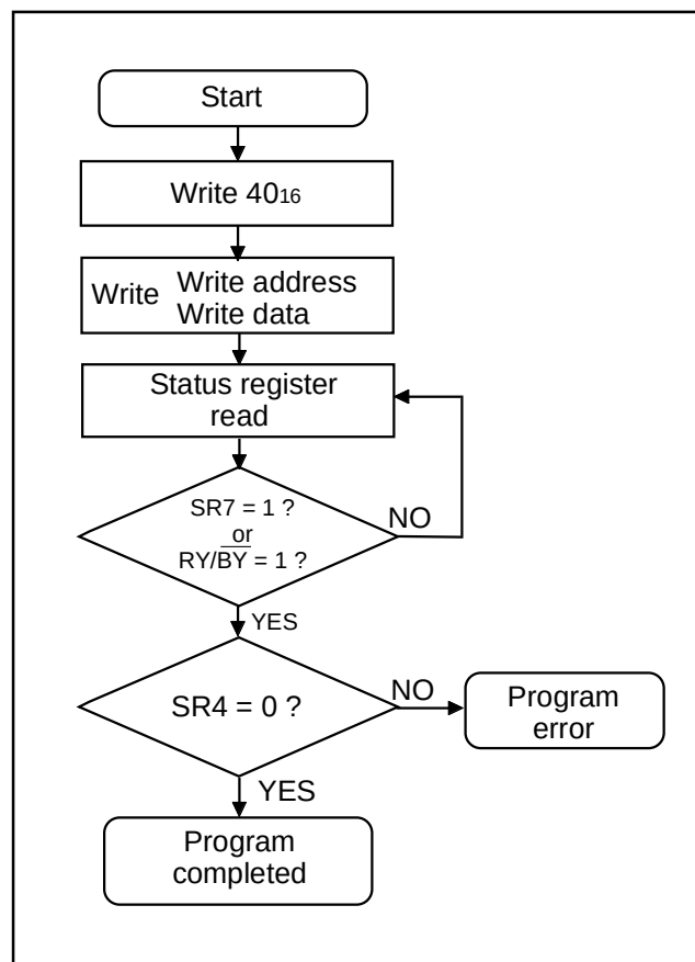
Fig. 149 Program flowchart
