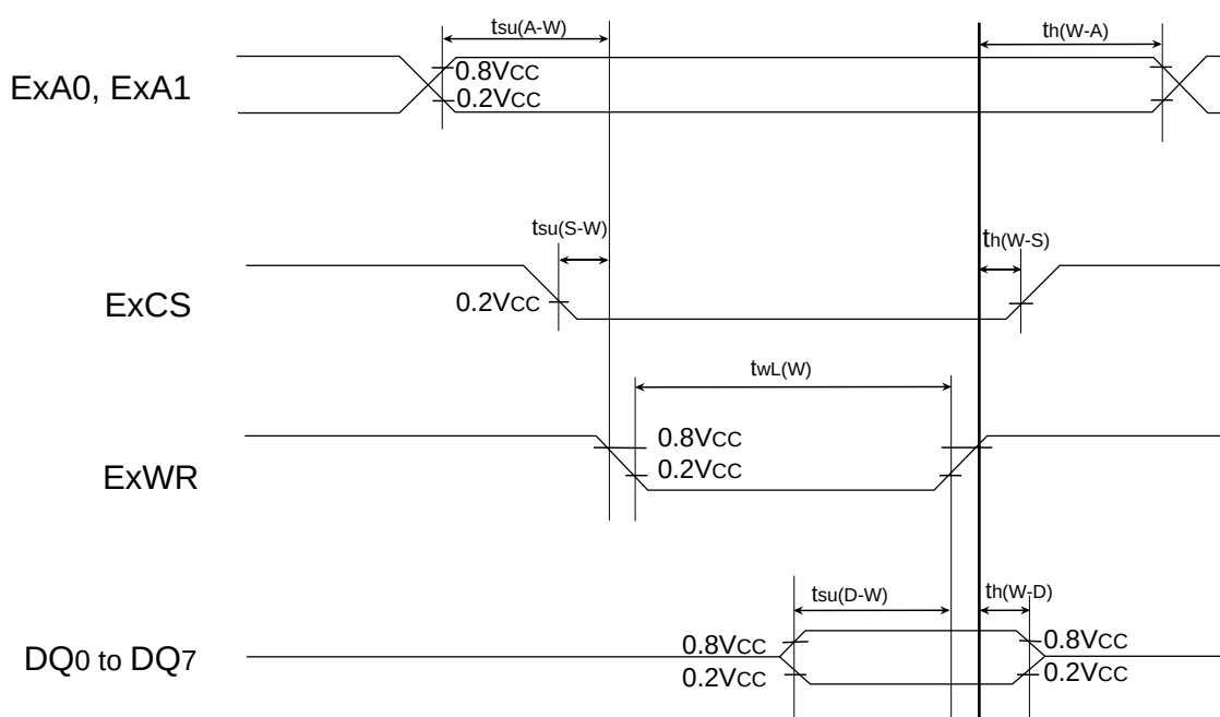
Fig. 172 Timing chart (2)
