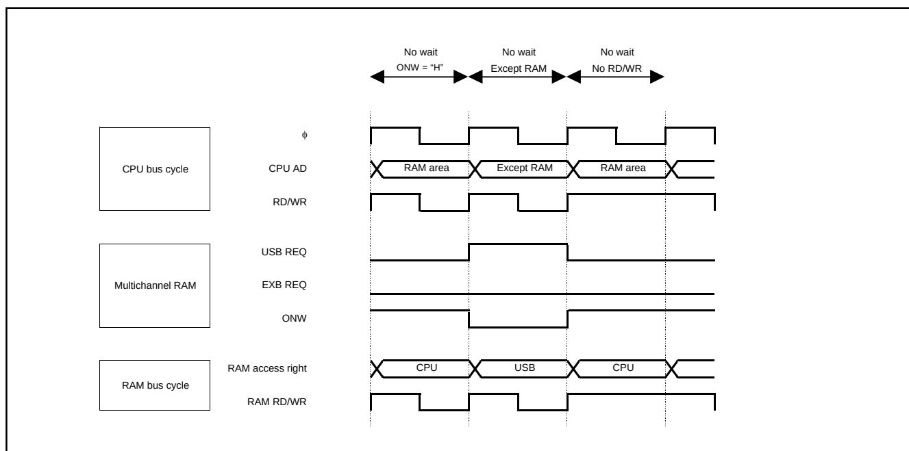
Fig. 129 Multichannel RAM timing diagram (no wait)
