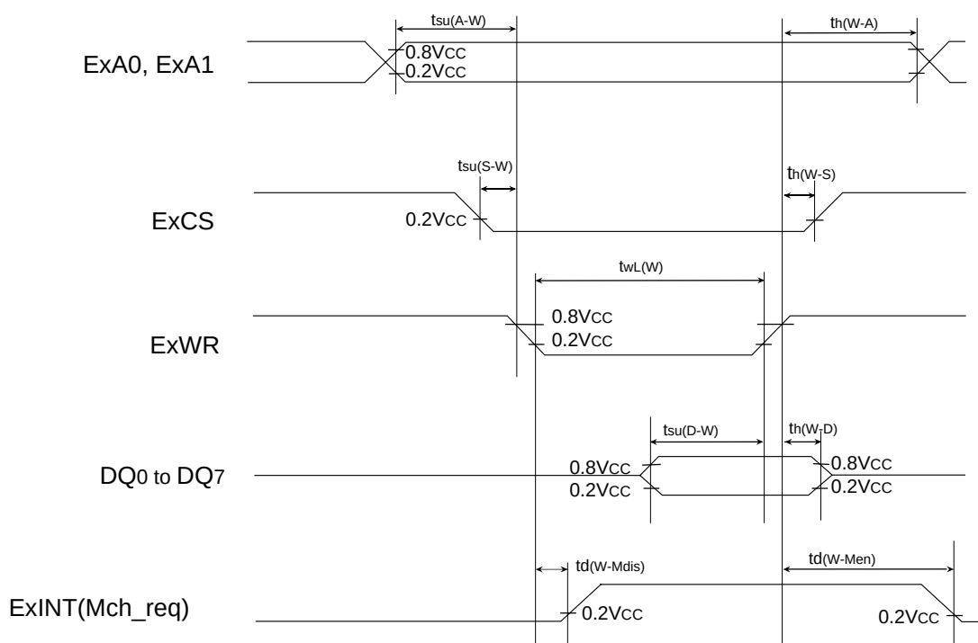
Fig. 173 Timing chart (3)
