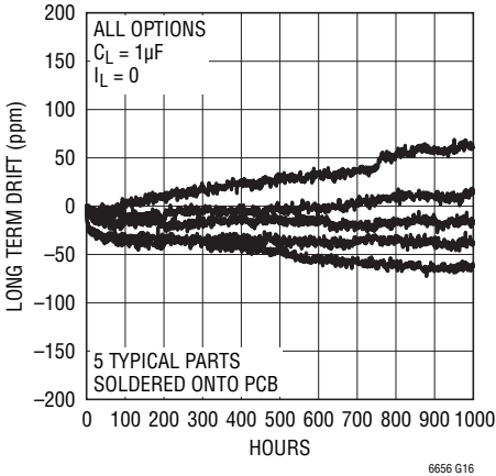
Long-Term Drift
