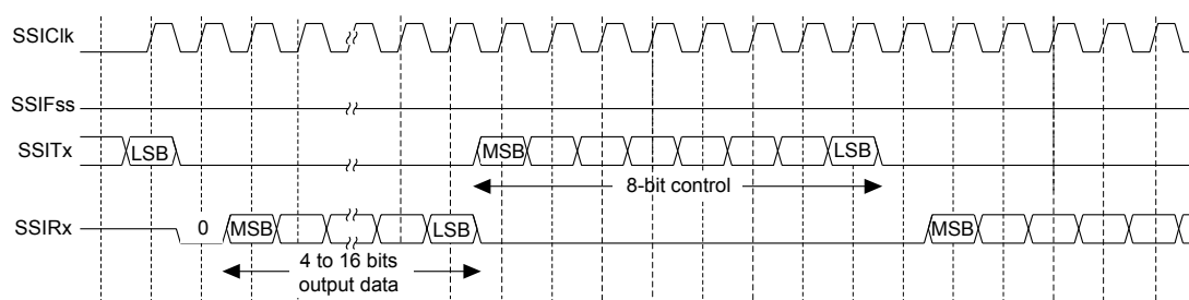
Figure 12-11. MICROWIRE Frame Format (Continuous Transfer)
