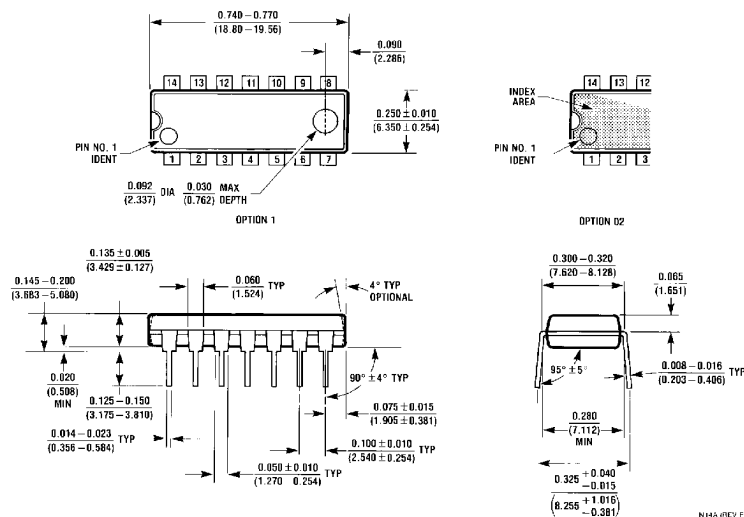
14-Lead Molded Dual-In-Line Package (N) Order Number DM74LS26N Package Number N14A
