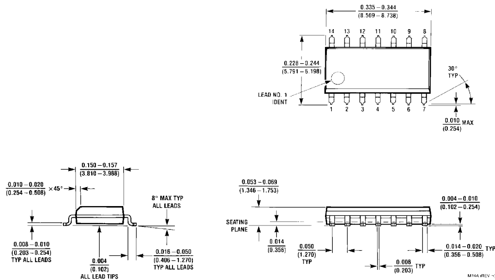
14-Lead Small Outline Molded Package (M) Order Number DM74LS26M Package Number M14A
