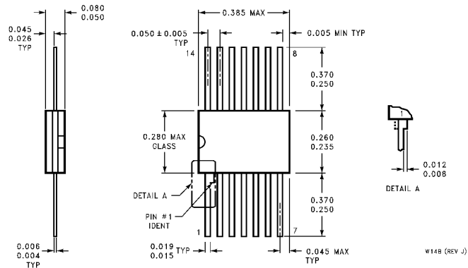
14-Lead Ceramic Flat Package (W) Order Number DM54LS26W Package Number W14B
