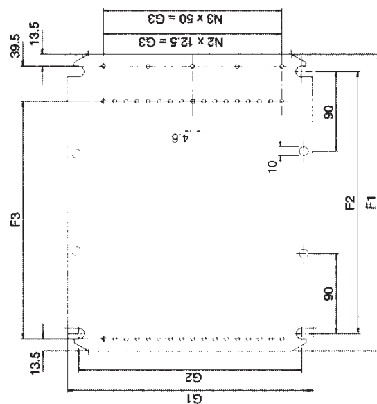
Montageplåt AE 1030/1031/1033/1034/1380/ 1039/1339
