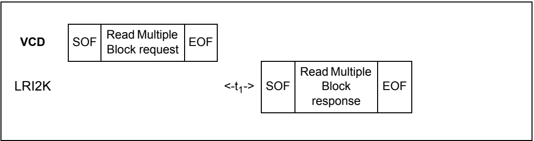
Figure 44. Read Multiple Block frame exchange between VCD and LRI2K
