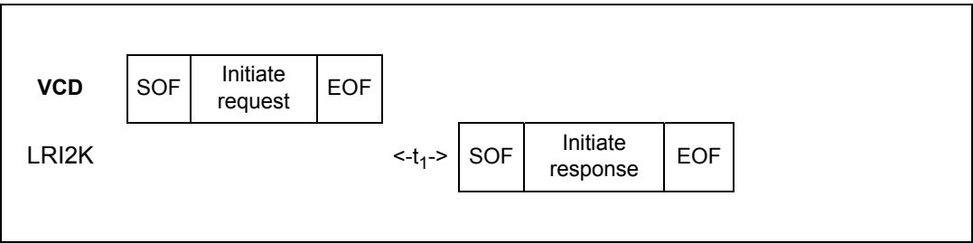
Figure 59. Initiate frame exchange between VCD and LRI2K
