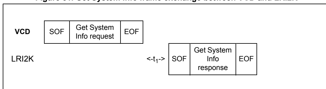
Figure 51. Get System Info frame exchange between VCD and LRI2K
