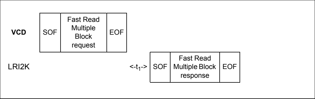
Figure 58. Fast Read Multiple Block frame exchange between VCD and LRI2K
