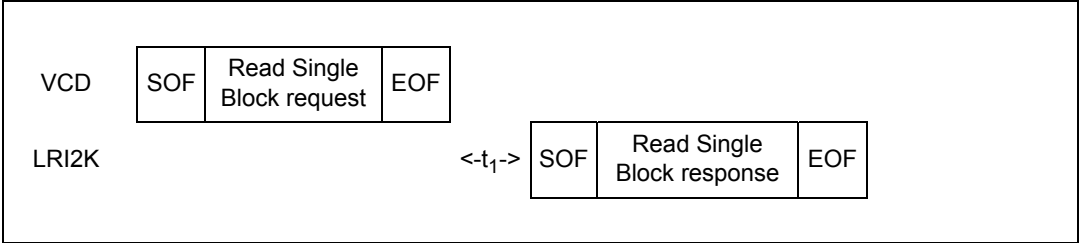
Figure 41. READ Single Block frame exchange between VCD and LRI2K
