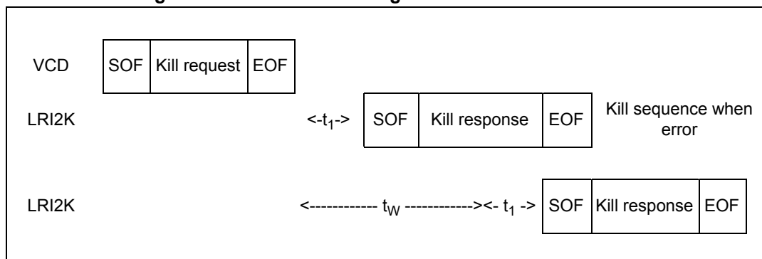
Figure 53. Kill frame exchange between VCD and LRI2K
