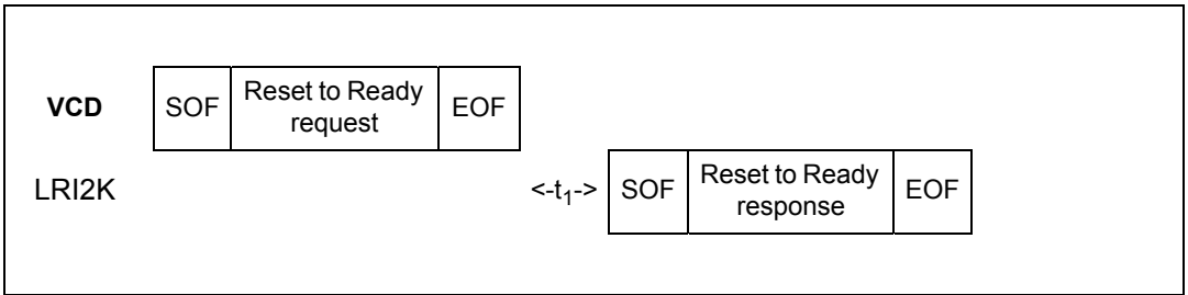
Figure 46. Reset to Ready frame exchange between VCD and LRI2K
