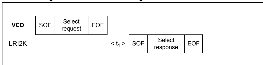
Figure 45. Select frame exchange between VCD and LRI2K
