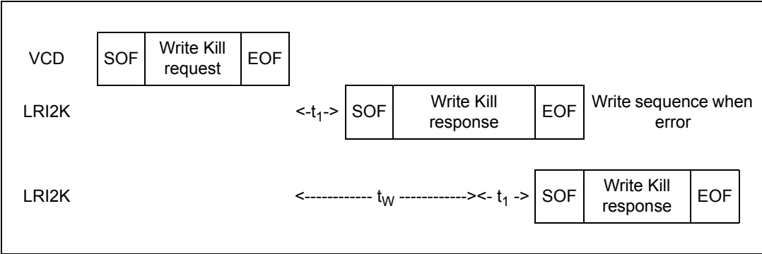
Figure 54. Write Kill frame exchange between VCD and LRI2K
