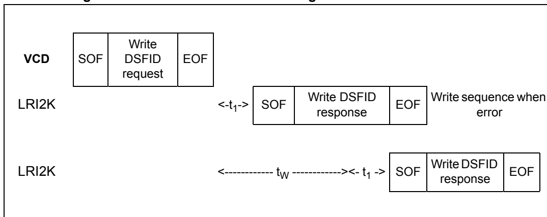
Figure 49. Write DSFID frame exchange between VCD and LRI2K
