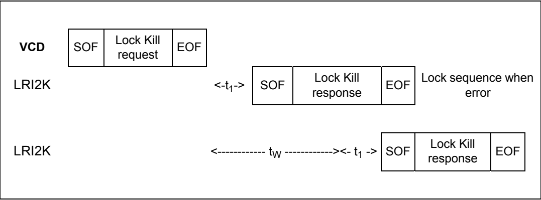
Figure 55. Lock Kill frame exchange between VCD and LRI2K
