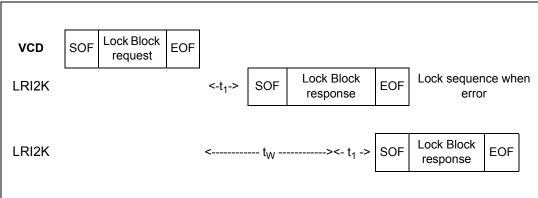
Figure 43. Lock Block frame exchange between VCD and LRI2K
