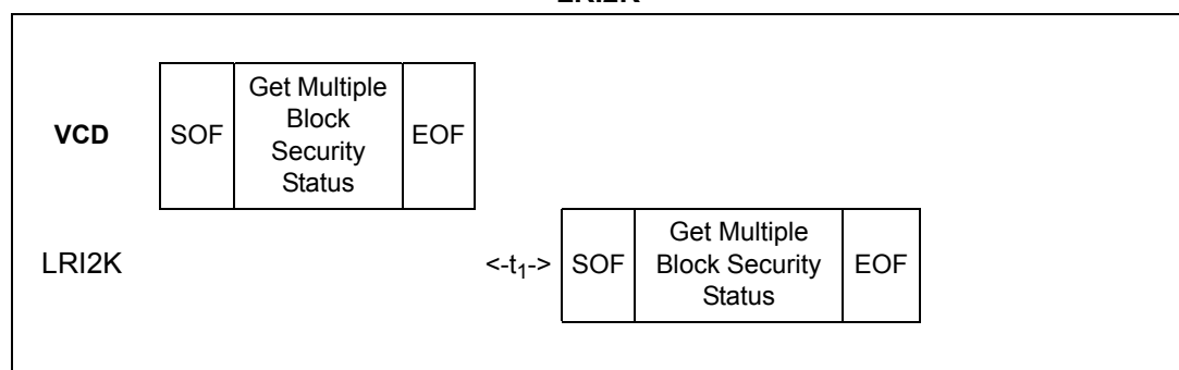
Figure 52. Get Multiple Block Security Status frame exchange between VCD and LRI2K
