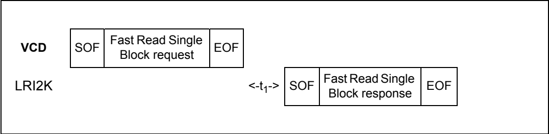
Figure 56. Fast Read Single Block frame exchange between VCD and LRI2K
