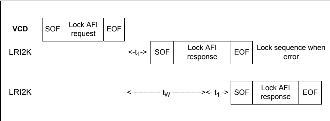
Figure 48. Lock AFI frame exchange between VCD and LRI2K
