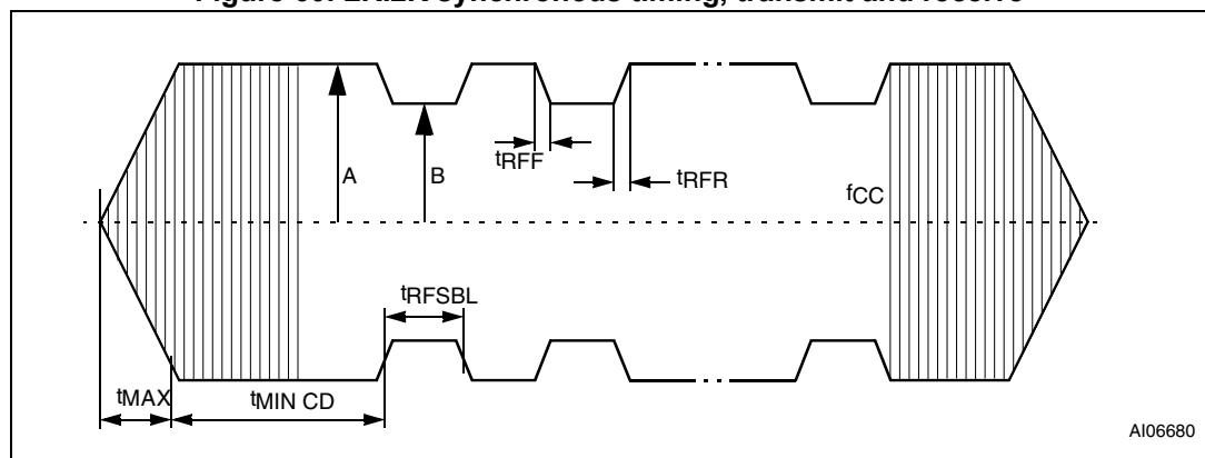
Figure 60. LRI2K synchronous timing, transmit and receive
