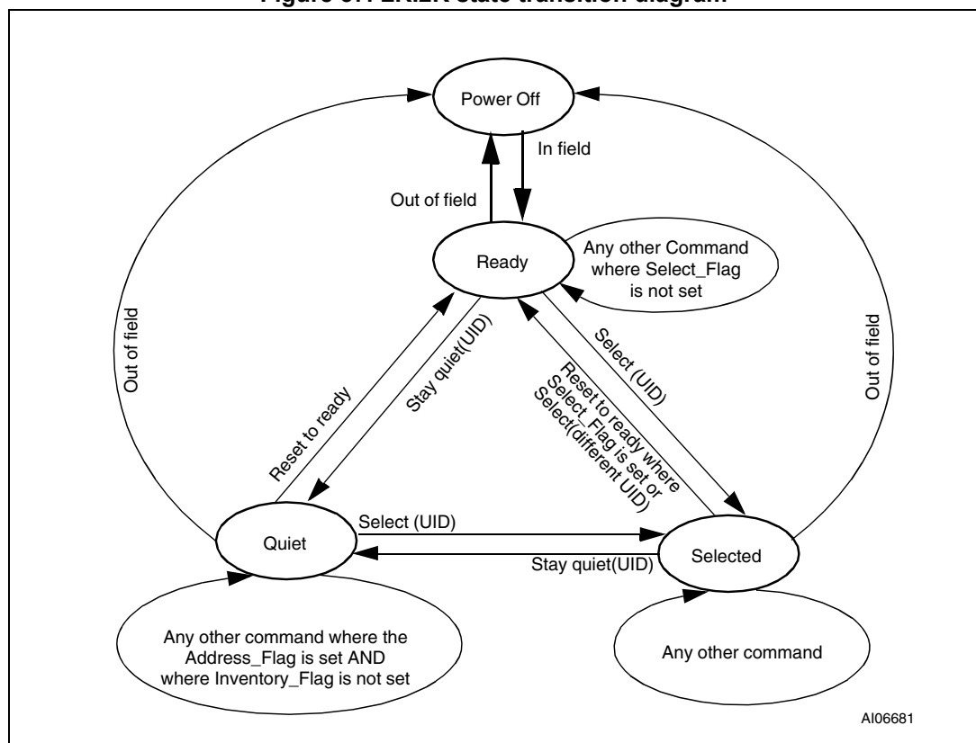
Figure 37. LRI2K state transition diagram
