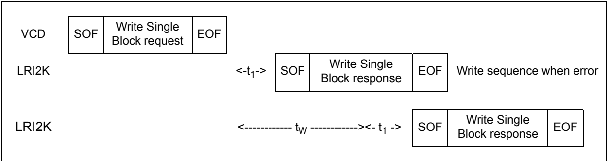
Figure 42. Write Single Block frame exchange between VCD and LRI2K
