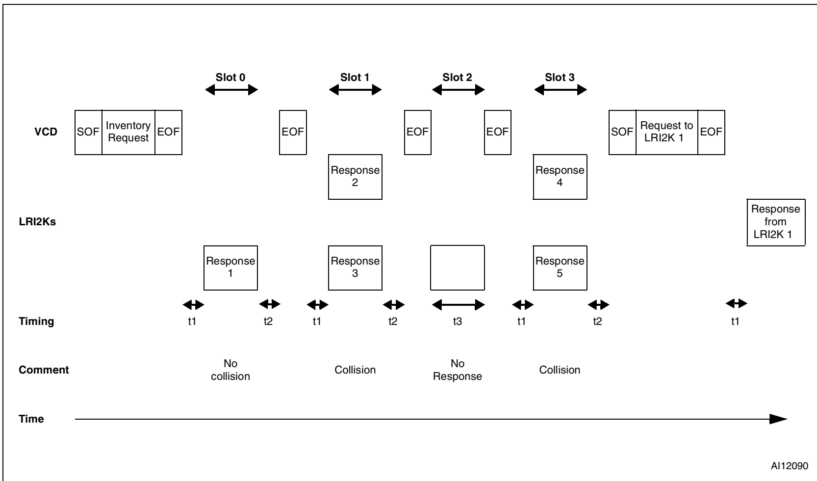
Figure 39. Description of a possible anticollision sequence
