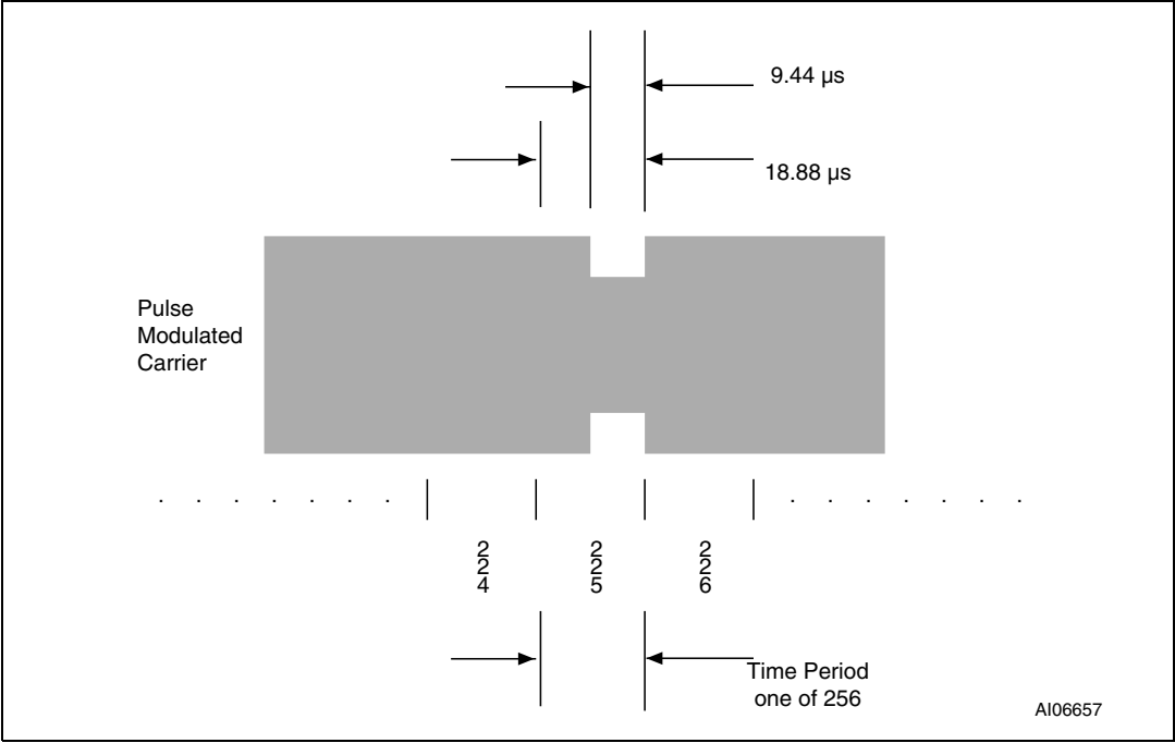
Figure 5. Detail of one time period
