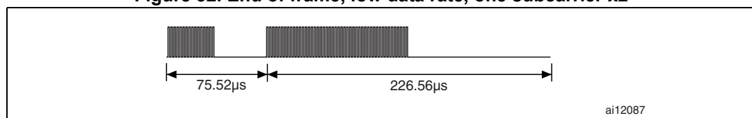
Figure 32. End of frame, low data rate, one subcarrier x2
