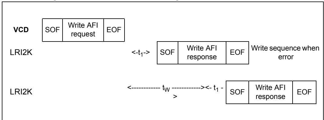
Figure 47. Write AFI frame exchange between VCD and LRI2K
