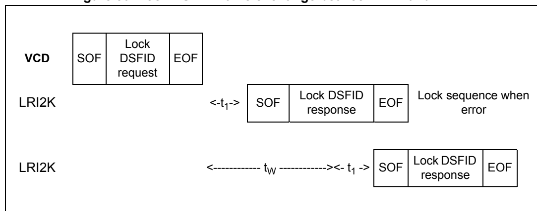
Figure 50. Lock DSFID frame exchange between VCD and LRI2K
