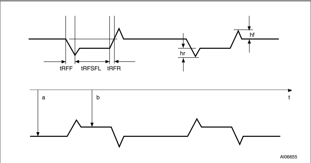
Figure 3. 10% modulation waveform
