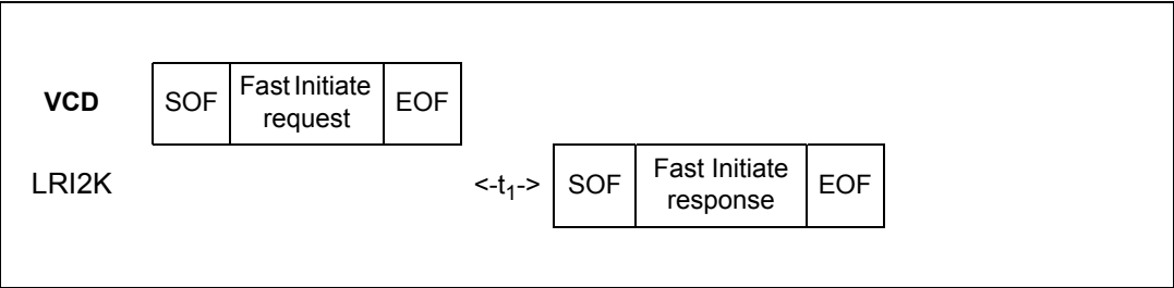
Figure 57. Fast Initiate frame exchange between VCD and LRI2K
