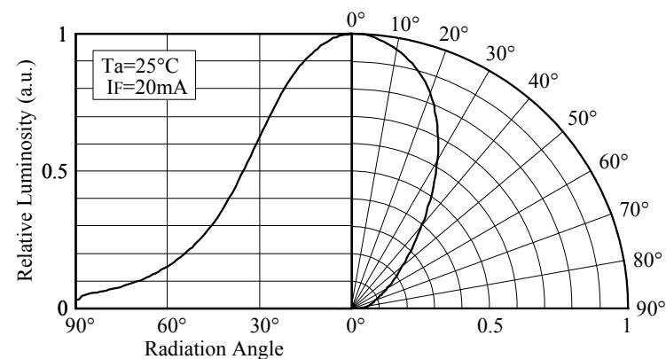
■ Directivity (NSPW315BS)
