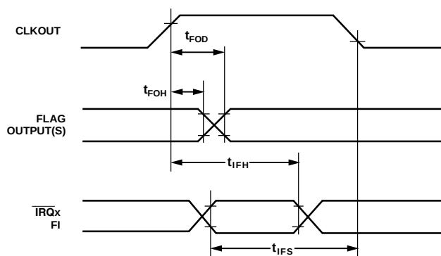
Figure 20. Interrupts & Flags
