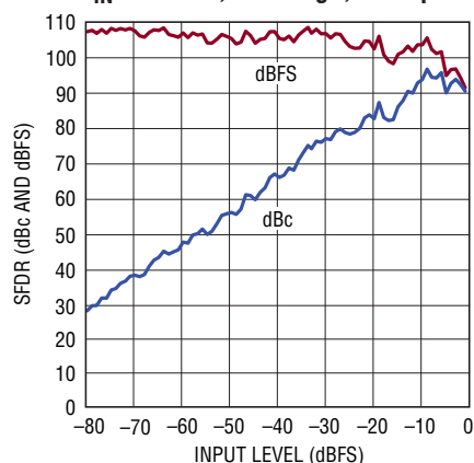
LTC2171-14: SFDR vs Input Level, f_{IN} = 70\text{MHz} , 2\text{V} Range, 40\text{Mpsps}
