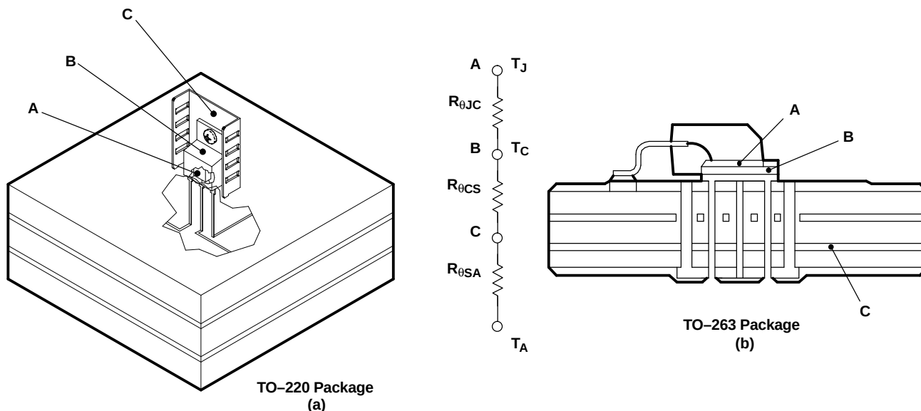
Figure 21. Thermal Resistances
