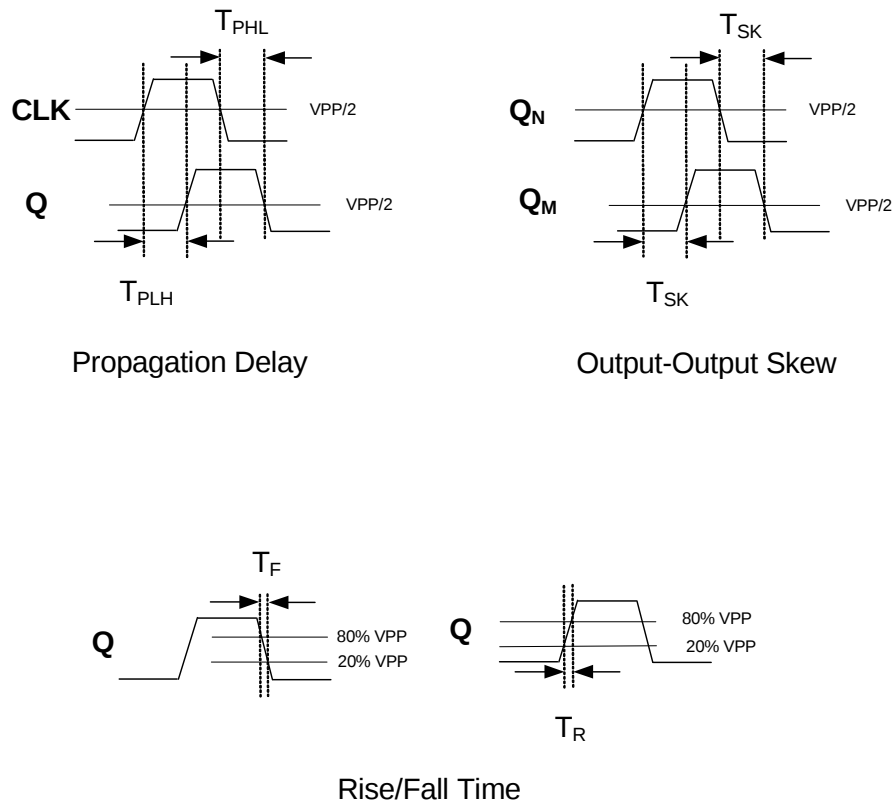
Figure 7. AC Waveforms
