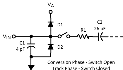
Figure 21. Equivalent Input Circuit
