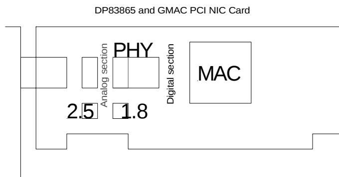
Figure 16. 1.8\text{ V} voltage regulator placement.
