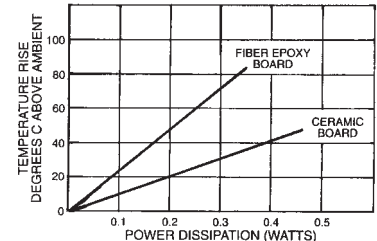
POWER DERATING
