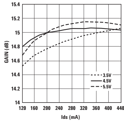
Figure 9. Gain vs. I_{ds} and V_{ds} at 2 GHz.
