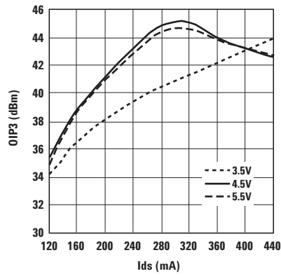
Figure 19. OIP3 vs. I_{ds} and V_{ds} at 2 GHz.
