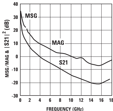
Figure 31. MSG/MAG & |S_{21}|^2 vs Frequency at 4.5V/280 mA.
