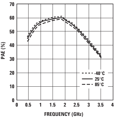
Figure 30. PAE vs. Temperature and Frequency at optimum P1dB.
