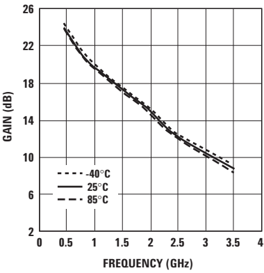
Figure 29. Gain vs. Temperature and Frequency at optimum P1dB.
