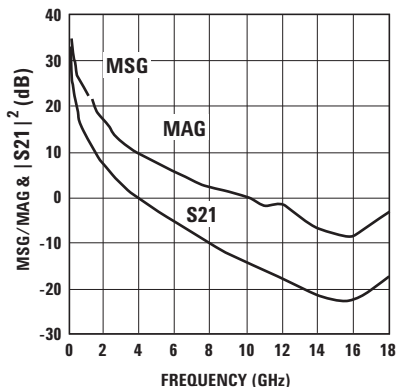
Figure 34. MSG/MAG & |S_{21}|^2 vs Frequency at 5.5V/280 mA.
