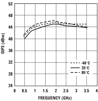
Figure 27. OIP3 vs. Temperature and Frequency at optimum P1dB.
