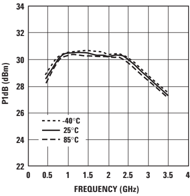
Figure 28. P1dB vs. Temperature and Frequency at optimum P1dB.
