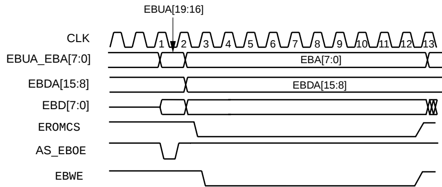
Figure 45. Flash Write from Expansion Bus Data Port
