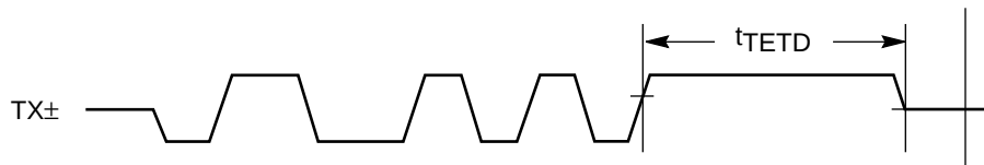
Figure 55 10 Mbps Transmit (TX±) Timing Diagram
