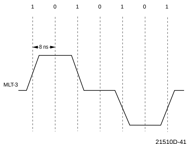
Figure 36. MLT-3 Waveform
