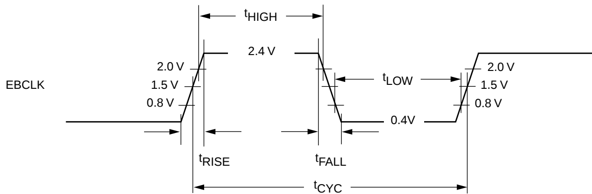
Figure 67 EBCLK Waveform
