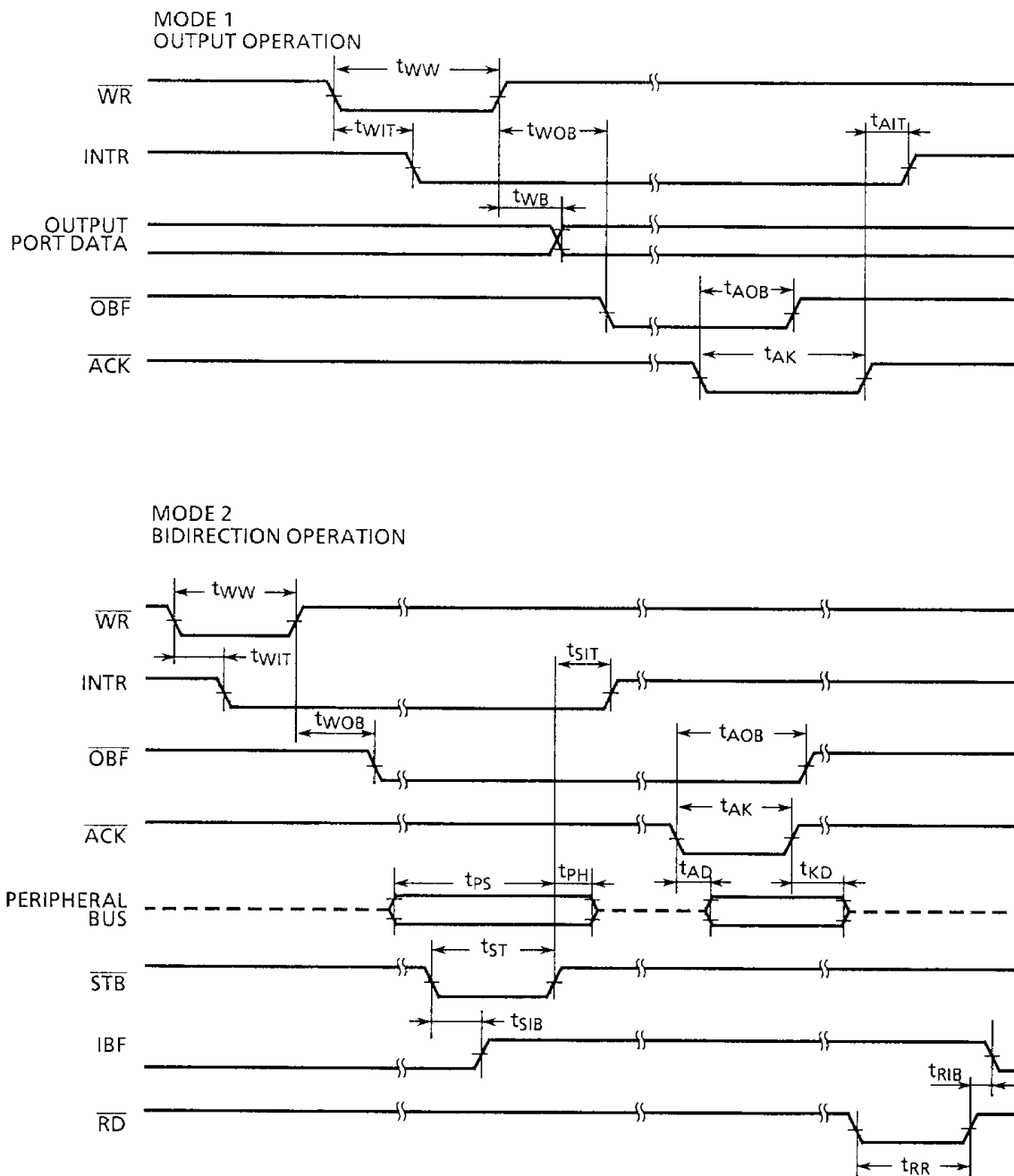
Figure 7.2 Timing diagram
