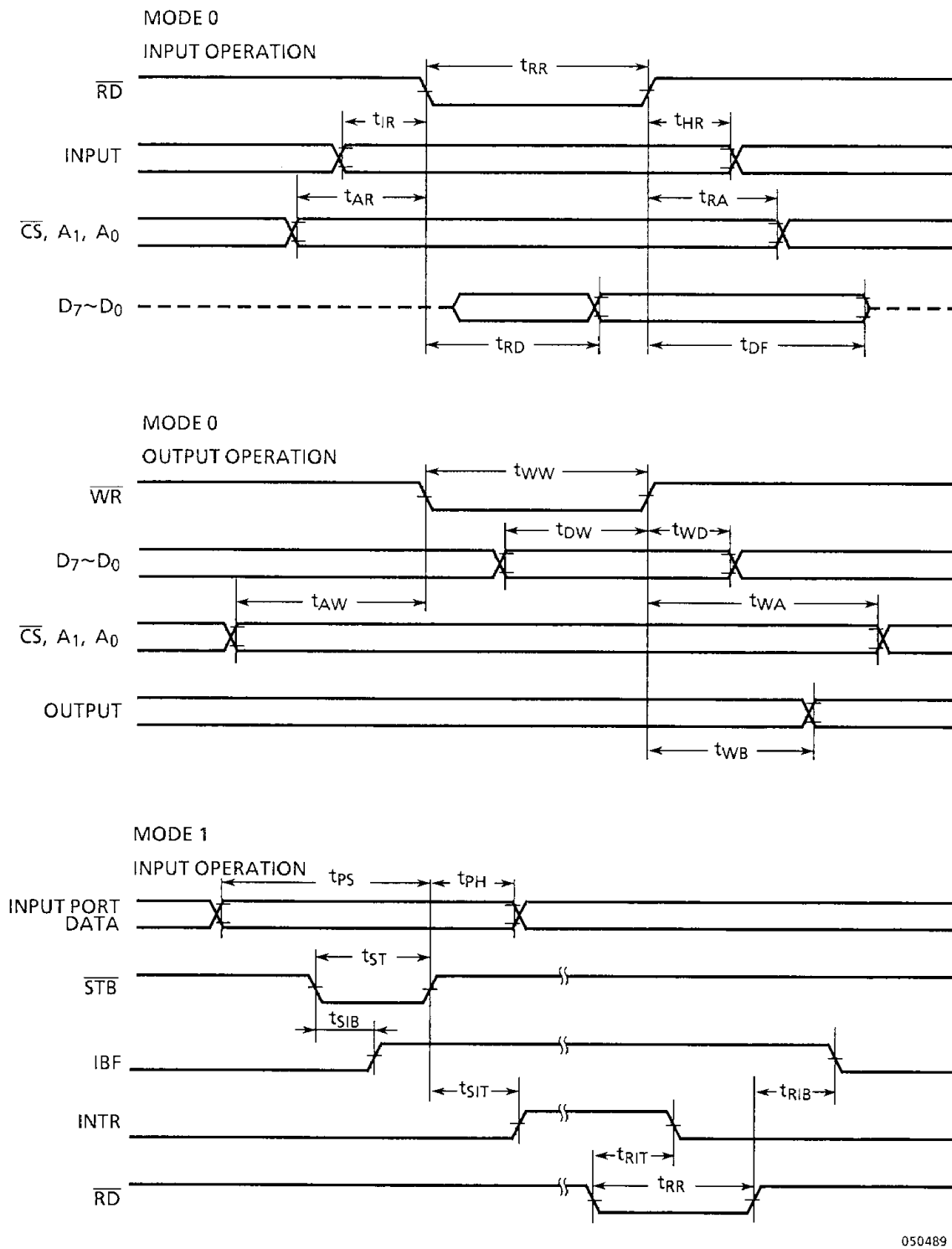
Figure 7.1 Timing diagram
