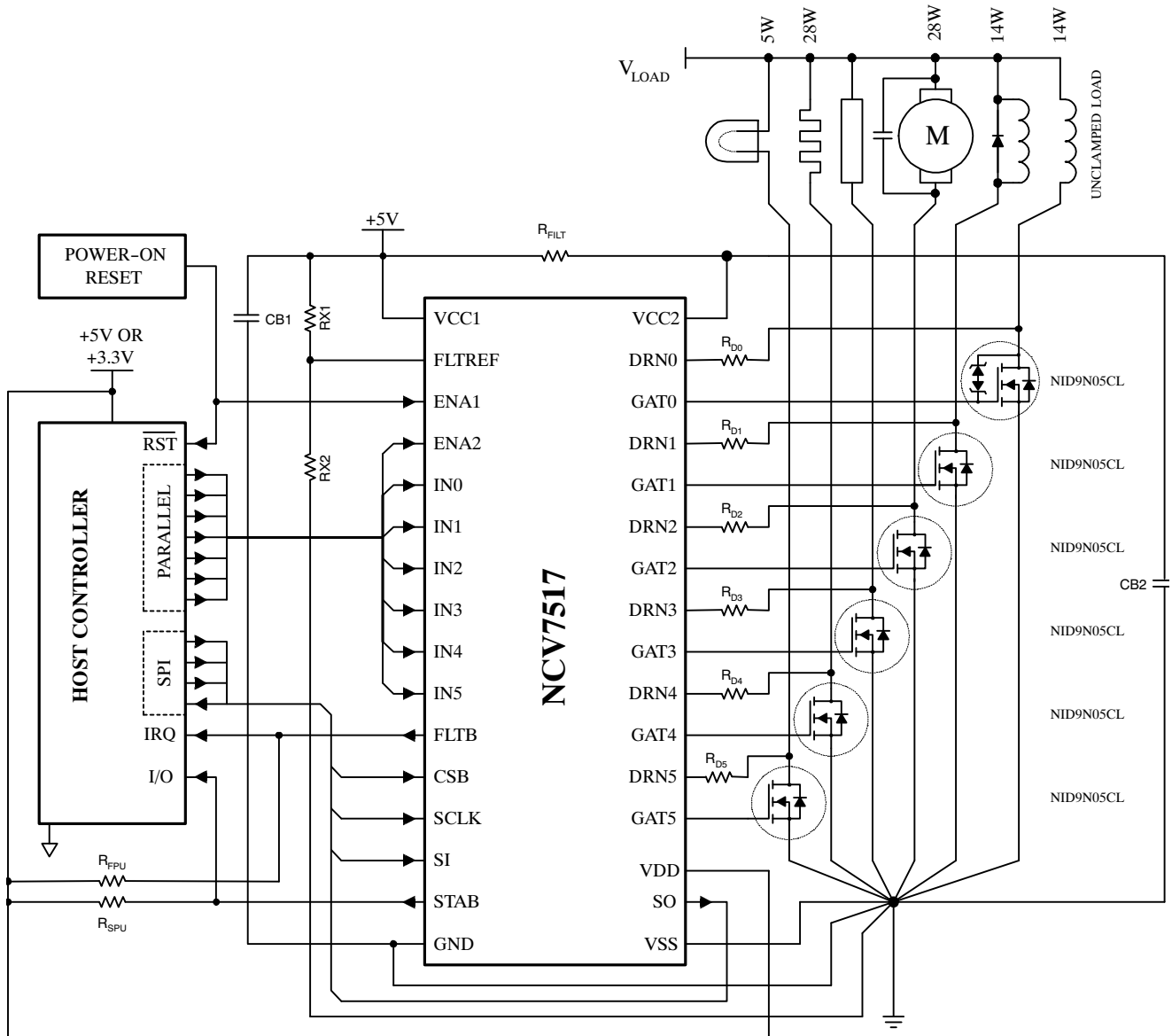
Figure 2. Application Diagram
