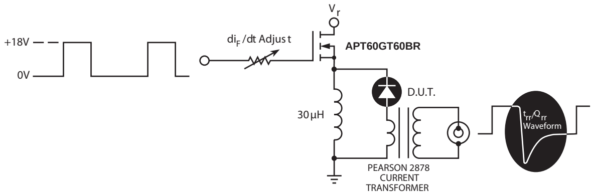
Figure 31. Diode Test Circuit
