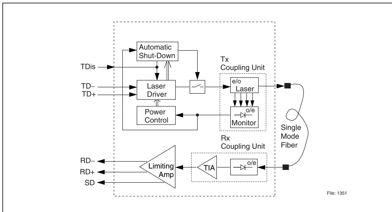
Figure 2 Functional Diagram
