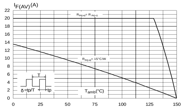
Figure 3: Average forward current versus ambient temperature ( \delta = 0.5 )
