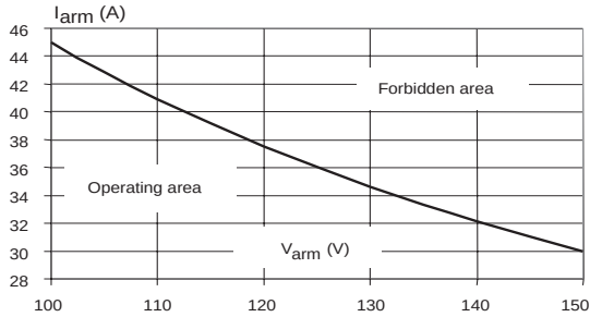
Figure 9: Reverse safe operating area ( t_p < 1 \mu\text{s} and T_J < 150^\circ\text{C} )
