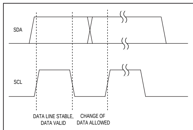
Figure 3. Bit Transfer
