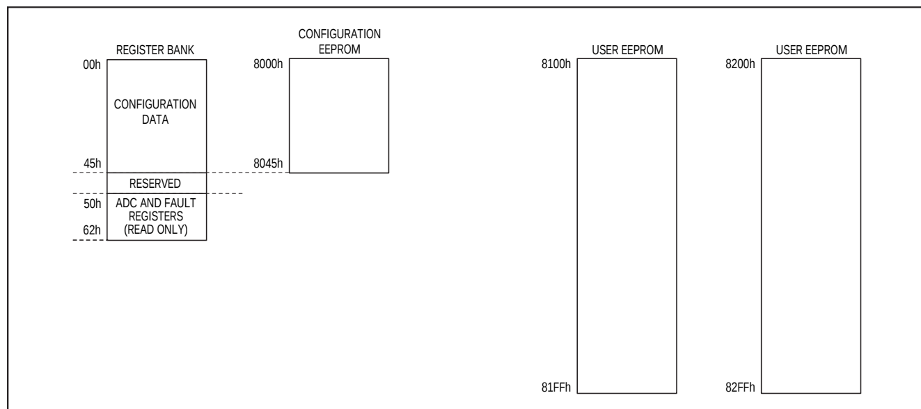
Figure 8. Memory Map
