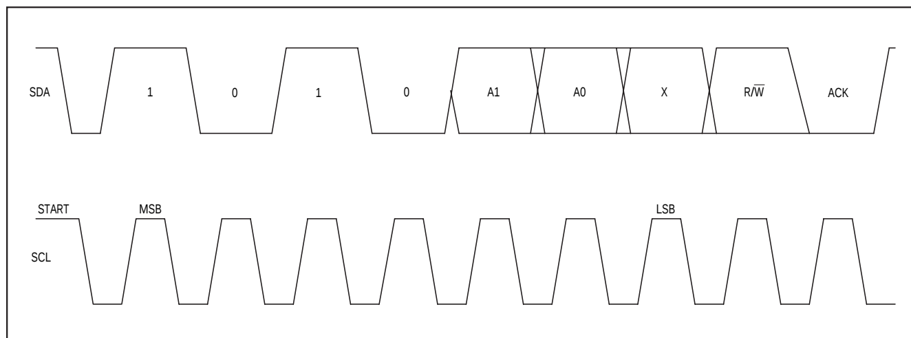
Figure 6. Slave Address
