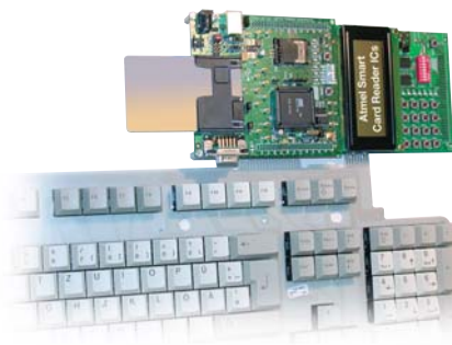
AT8xC5122/23 Development Board
