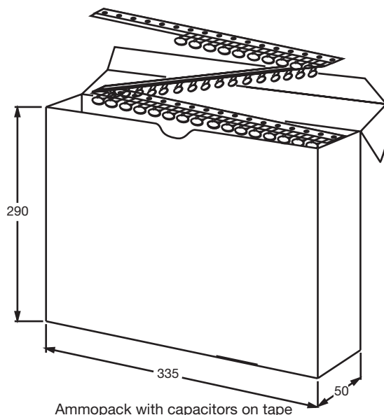
Ampmopack with capacitors on tape
