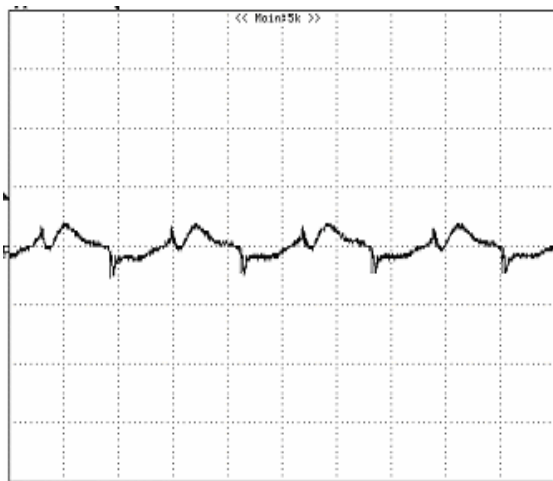
Figure 14: Output voltage ripple at nominal input voltage and rated load current ( I_o=25\text{A} ) (50 mV/div, 1us/div) Load capacitance: 1\mu\text{F} ceramic capacitor and 10\mu\text{F} tantalum capacitor. Bandwidth: 20 MHz. Scope measurements should be made using a BNC cable (length shorter than 20 inches). Position the load between 51 mm to 76 mm (2 inches to 3 inches) from the module
