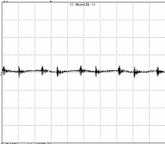
Figure 12: Input reflected ripple current, i_s , through a 12\mu\text{H} source inductor at nominal input voltage and rated load current (20 mA/div, 1us/div)
