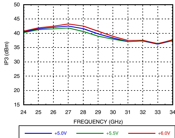
Output IP3 vs. Supply Voltage, Pout/Tone = +22 dBm
