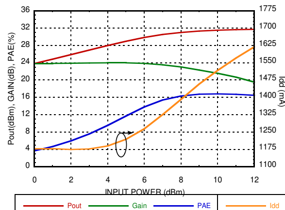
Power Compression @ 29 GHz
