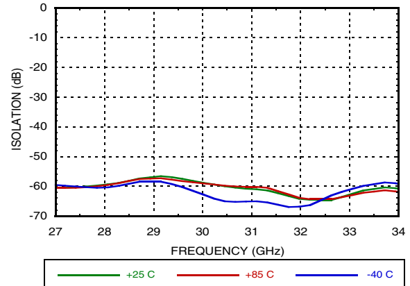
Reverse Isolation
