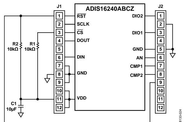
Figure 25. Electrical Schematic
