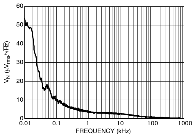
Figure 40. Output Voltage Noise, 1.2 V Version, V_{IN} = 2.2\text{ V} , I_{OUT} = 30\text{ mA}
