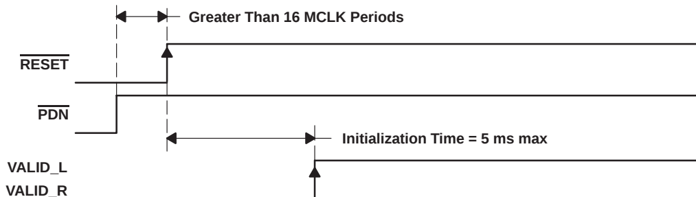
Figure 2. Power-Up Timing ( \overline{\text{PDN}} Preceding \overline{\text{RESET}} )
