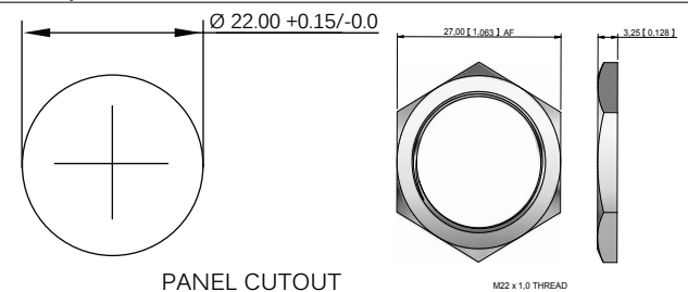
PANEL CUTOUT
