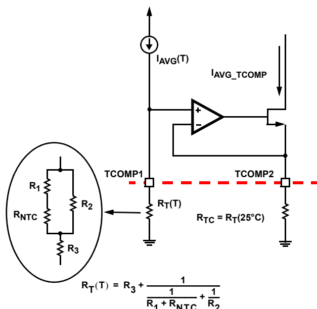
FIGURE 5. AVERAGE CURRENT TEMPERATURE COMPENSATION
