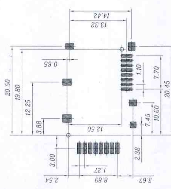
RECOMMEND P.C.B LAYOUT (ALL TOLERANCES:0.03mm)
