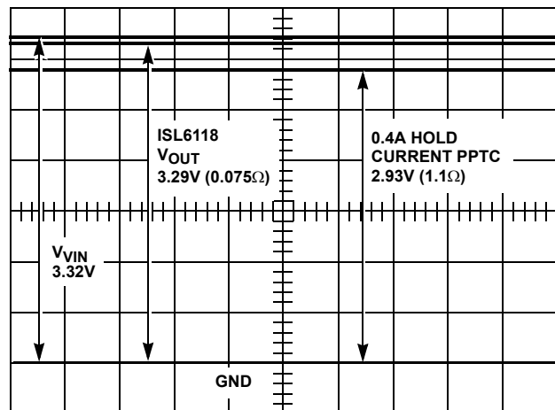
FIGURE 11. ISL6118 vs PPTC INTO 8.2Ω LOAD
