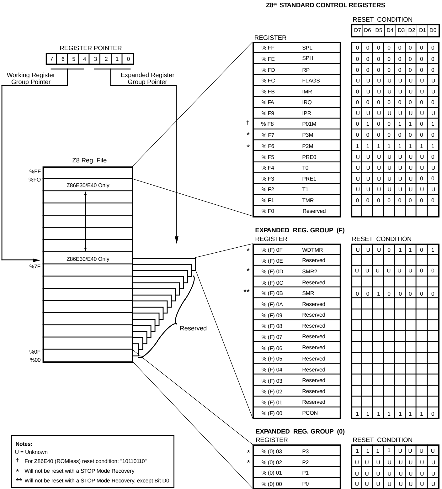
Figure 26. Expanded Register File Architecture
