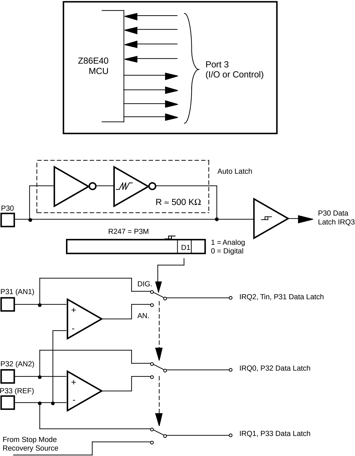
Figure 21. Port 3 Configuration
