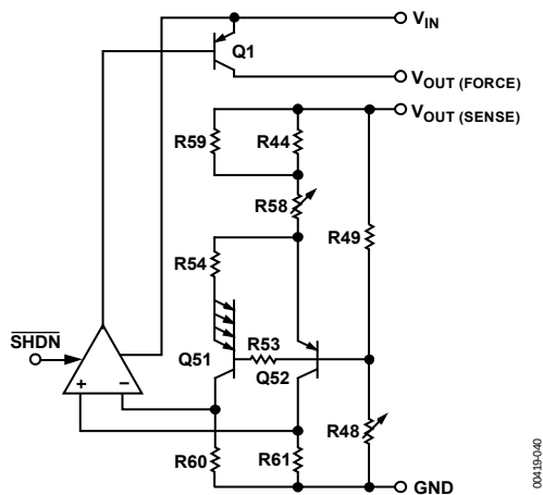
Figure 39. Simplified Schematic
