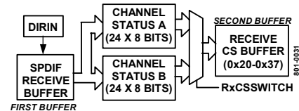
Figure 29. Channel Status Buffer
