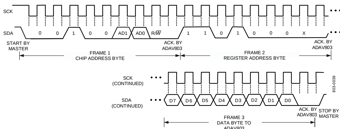
Figure 38. Writing to the ADAV804 in I²C
