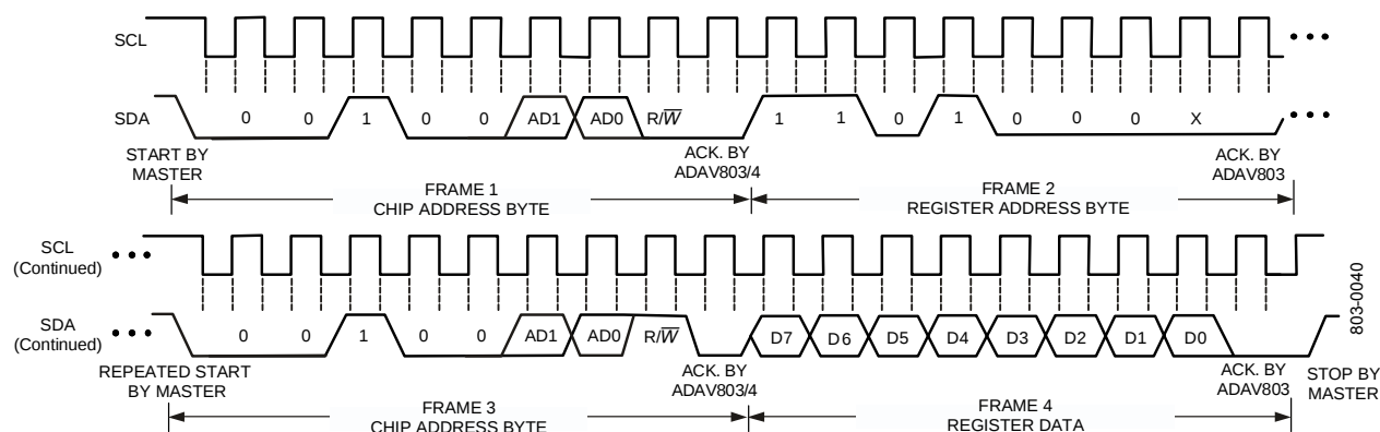
Figure 39. Reading From the DAC Left Volume Register in I²C
