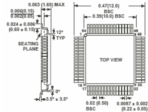
Figure 40. 64-Lead Plastic Quad Flatpack [LQFP] (ST-64) Dimensions shown in inches and (millimeters)
