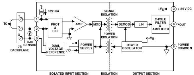
Figure 1. 7B47 Functional Block Diagram
