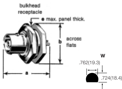
Bulkhead Receptacles 82-515
