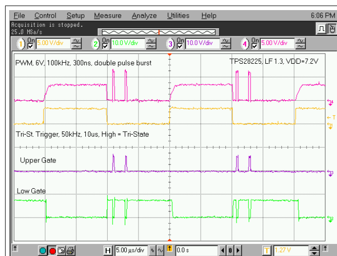
Figure 21. 6-V Amplitude PWM Pulse (TPS28225 example)
