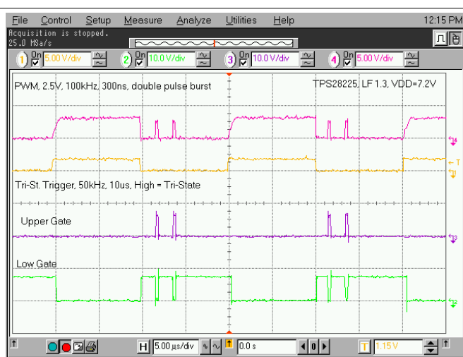
Figure 22. 2.5-V Amplitude PWM Pulse (TPS28225 example)
