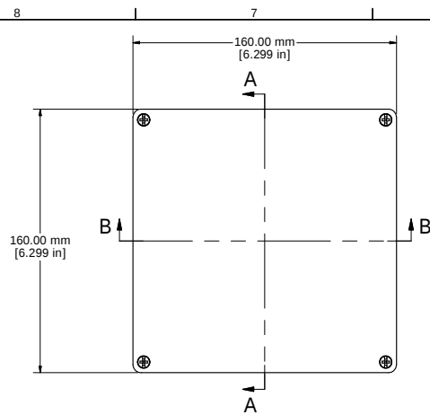
ASSEMBLY
