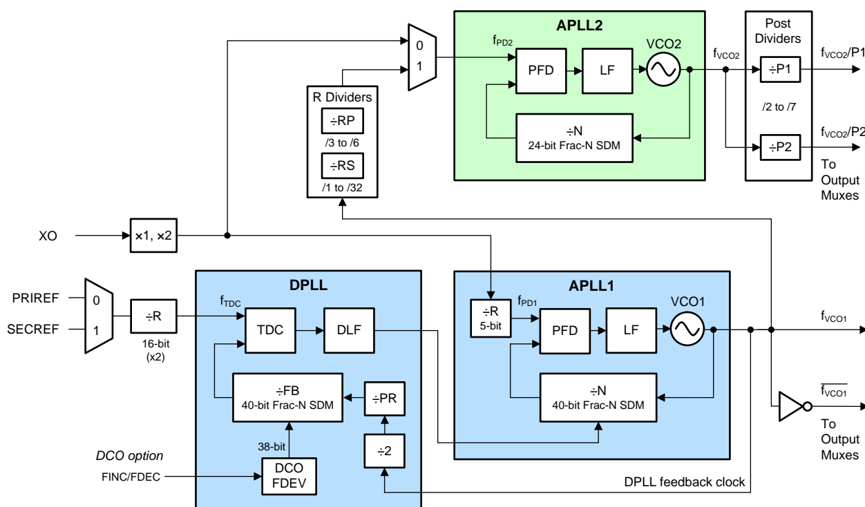
Figure 23. PLL Architecture
