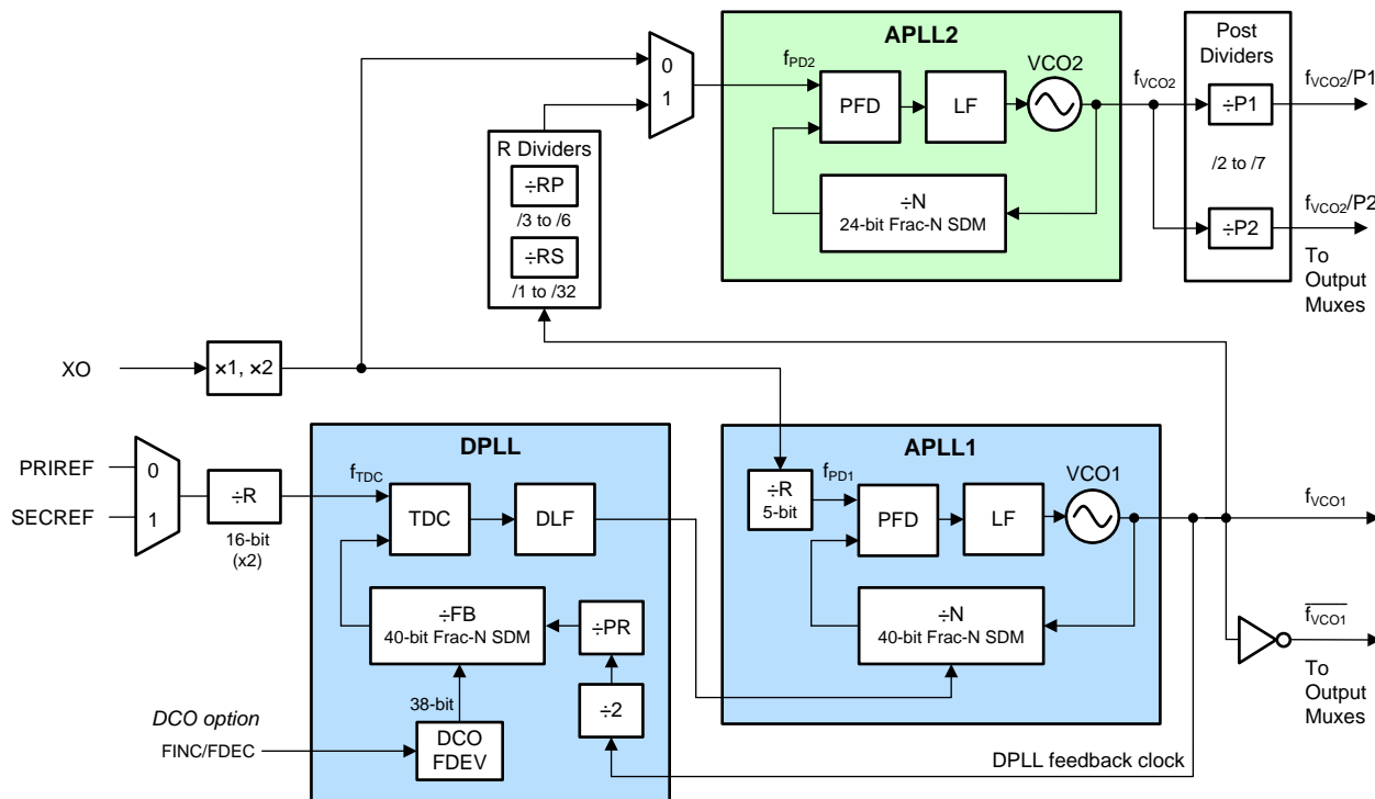
Figure 43. PLL Architecture
