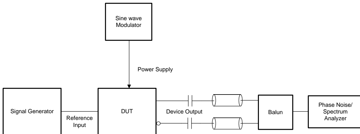
Figure 20. HCSL Output Phase Noise Test Configuration
