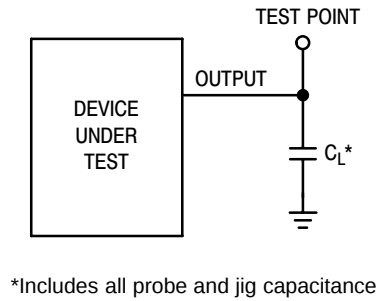
Figure 7. Test Circuit
