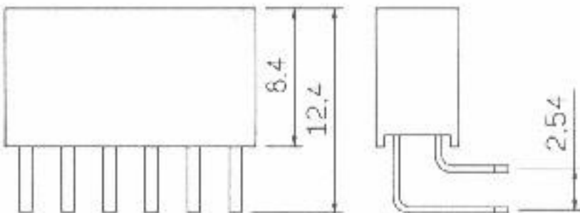
Right Angle Type Double Row
