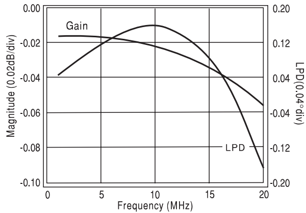
Gain Flatness & Linear Phase Deviation
