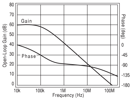
Open-Loop Gain & Phase
