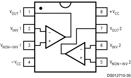
Pinout DIP & SOIC
