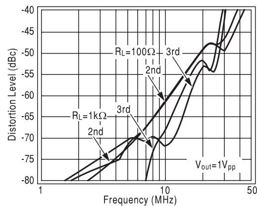
2nd and 3rd Harmonic Distortion
