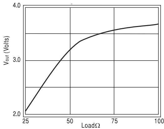
Maximum Output Voltage vs. Load
