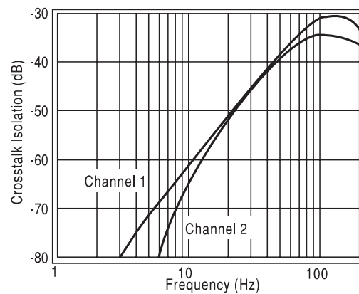
Channel-to-Channel Crosstalk
