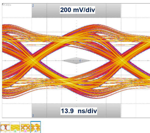
Figure 5. HDMI2.1 - 12 Gbps per channel without device (with worst cable model), 8dB CTLE and 25 mV DFE
