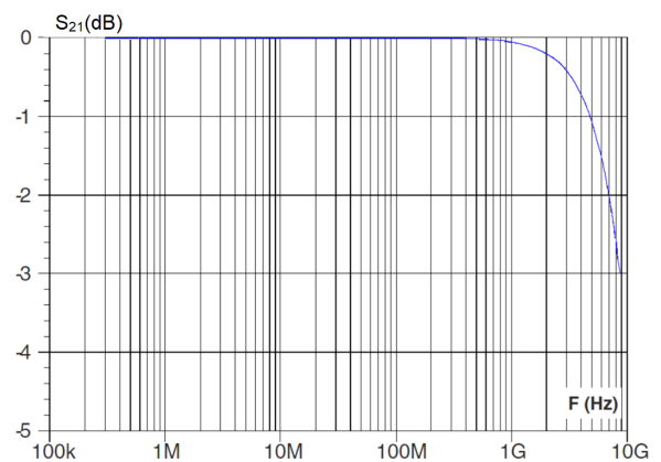
Figure 4. S_{21} attenuation
