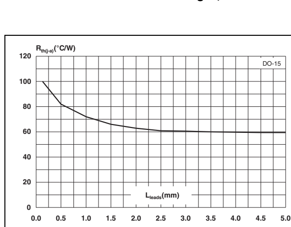
Figure 15. Thermal resistance junction to ambient versus lead length, DO-15
