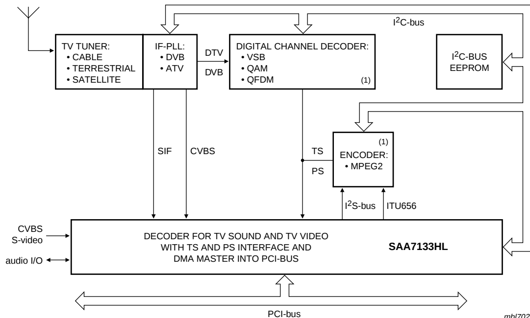
Fig 1. Application diagram for capturing live TV video and audio streams in the PC, with optional extensions for DTV and DVB capture and MPEG encoding for time shift viewing
