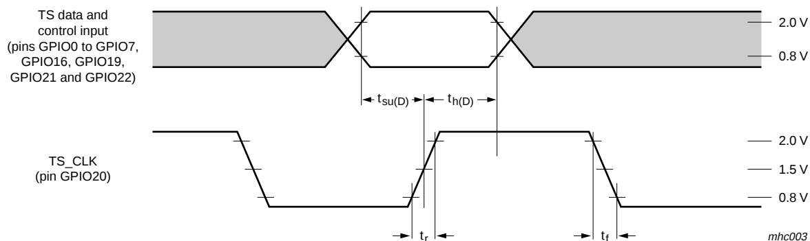
Fig 15. Data input timing (TS data and control inputs)
