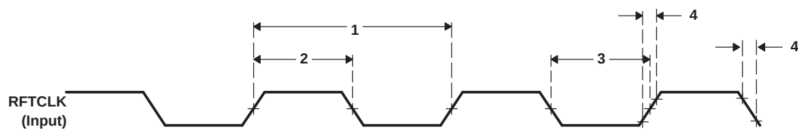
Figure 7-52. RFTCLK Timing [GMII Operation]
