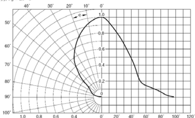
Radiation Characteristic
